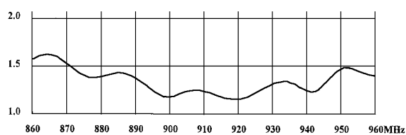
VSWR v Freq (MHz)
