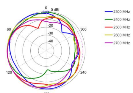
Elevation: 2300 – 2700 MHz
