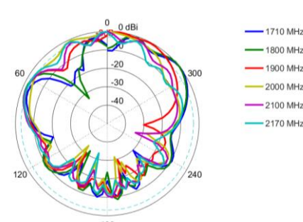
Elevation: 1710 – 2170 MHz
